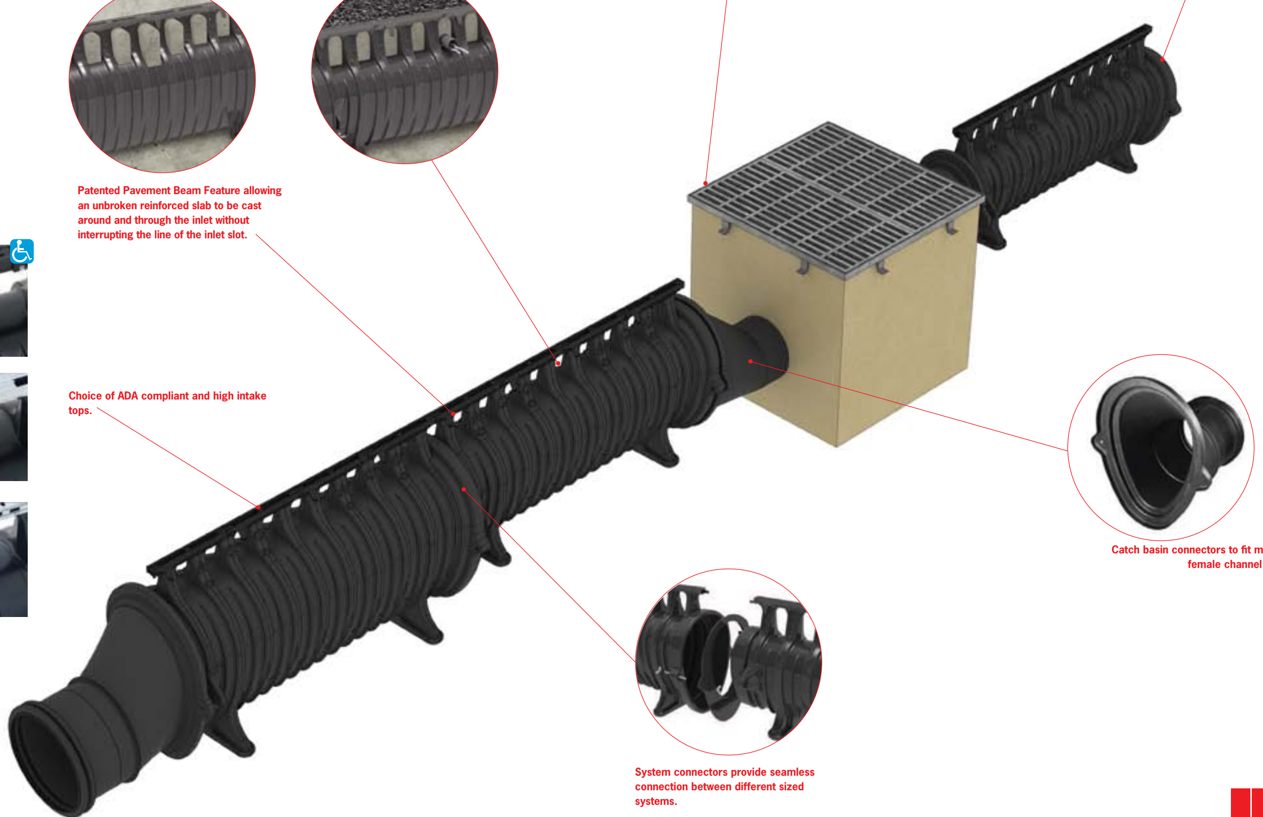
Q-Guard ductile iron ADA compliant tops
